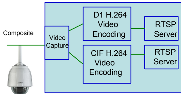
H.264 Dual Video Encoding
