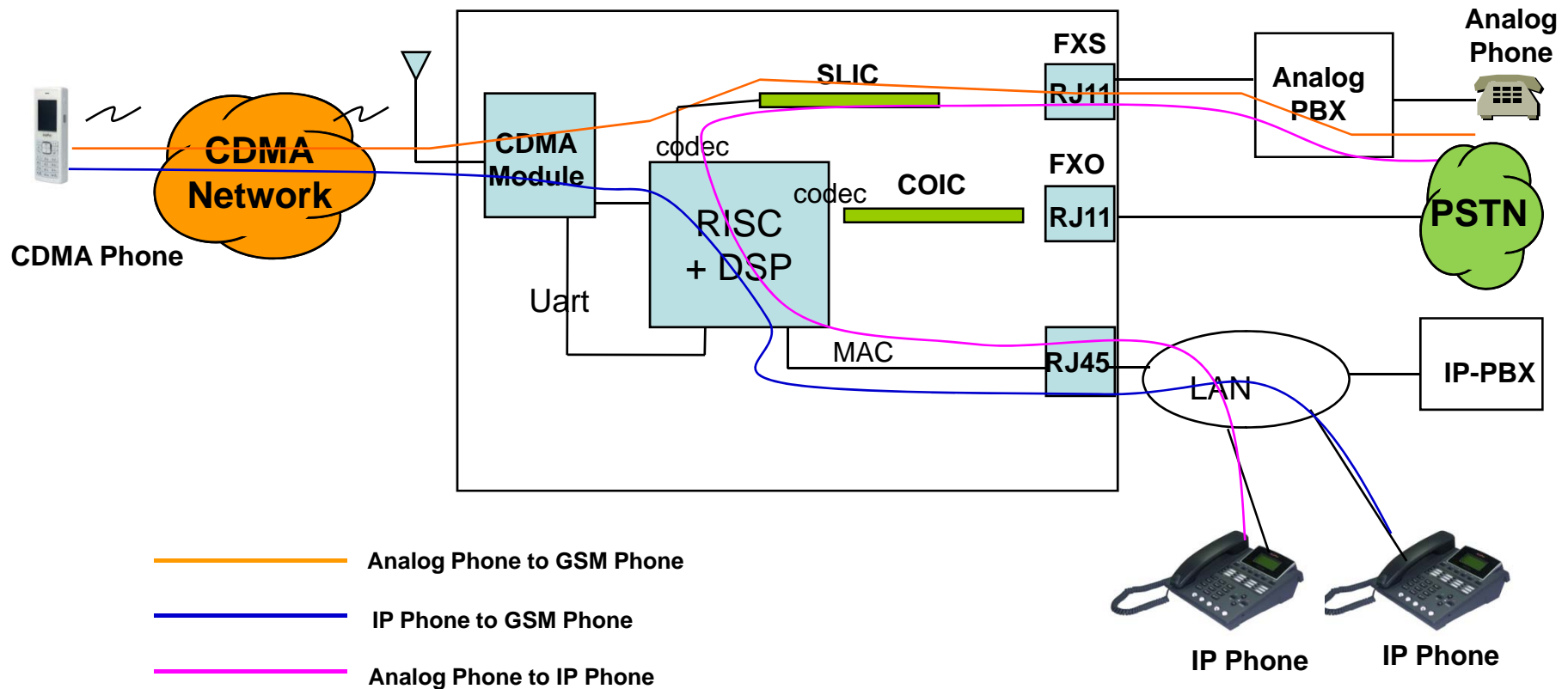
AP-CD701E CDMA Gateway Internal H/W Block Diagram
