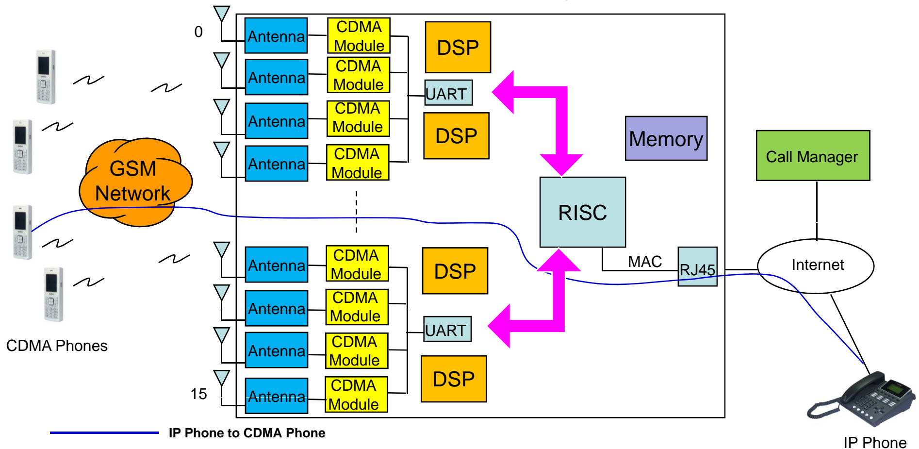
AP-CD816 Internal H/W Block Diagram
